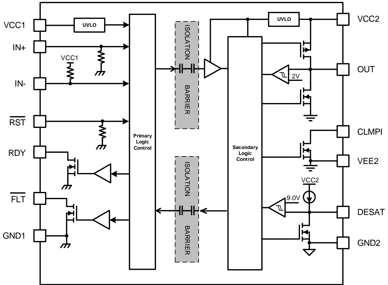
Figure 2. SiLM5851NH Block Diagram
