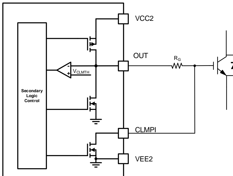
Figure 33. Active Miller Clamp
