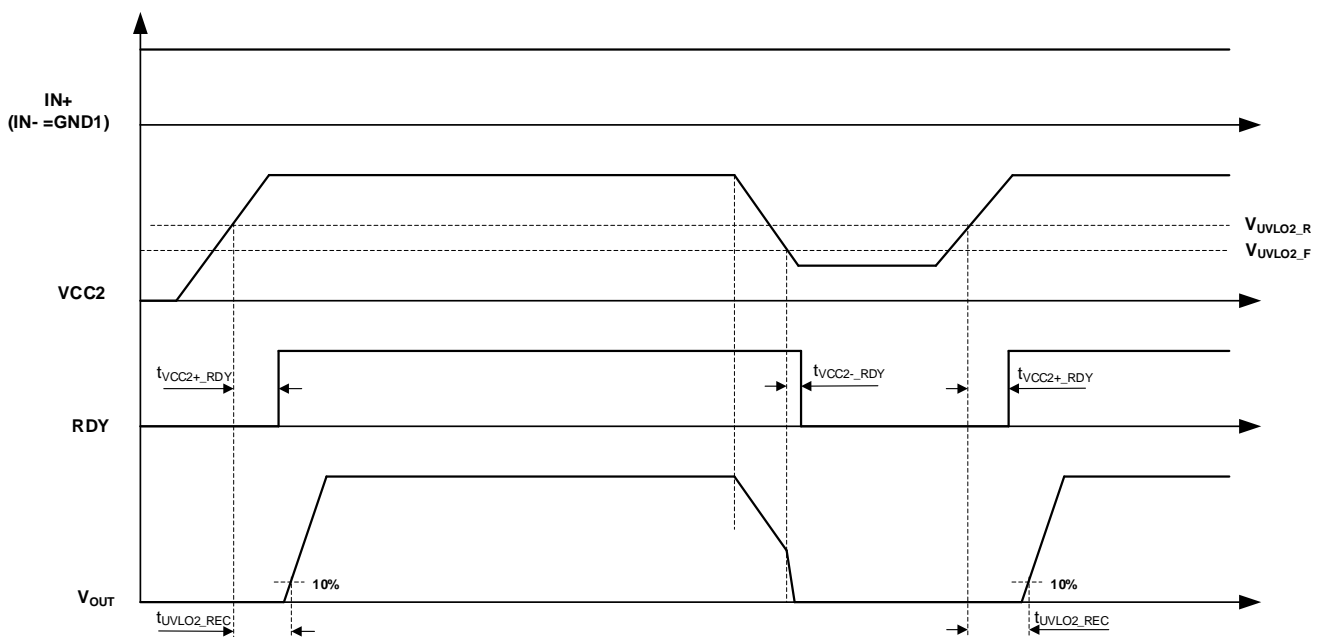
Figure 30.VCC2 UVLO Protection Timing
