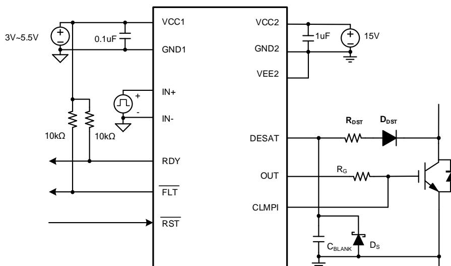
Figure 1. SiLM5851NH Application Circuit to Driver IGBT
