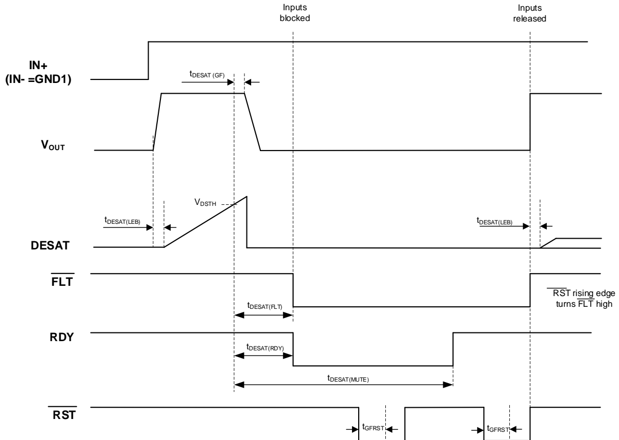
Figure 31. \overline{FLT} , \overline{RDY} and \overline{RST} Timing Diagram
